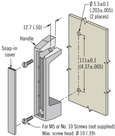
Front Install Concealed
