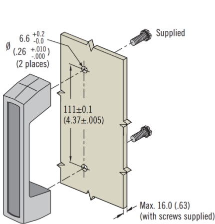
Rear Install Concealed
